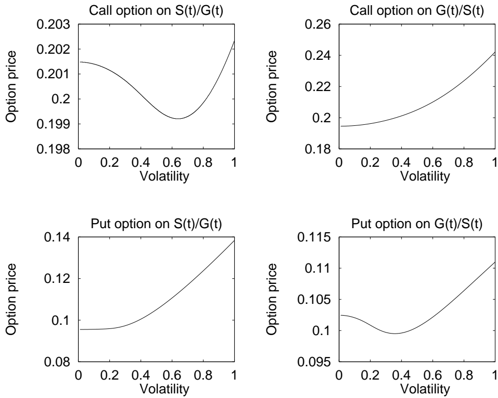
Figure 4: Geometric Australian option prices as a function of volatility ( \sigma ). The exercise price is K = 0.8 for calls and K = 1.1 for puts. The other parameter values are: r = 0.1 , q = 0.03 , T = 0.1 , and n = \infty .
